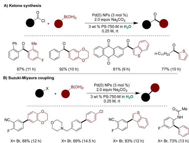
Scheme 34 Ligand-free ultrasmall Pd(0) NPs for, (A) biaryl ketone synthesis, and (B) Suzuki–Miyaura couplings in aqueous micellar medium.
