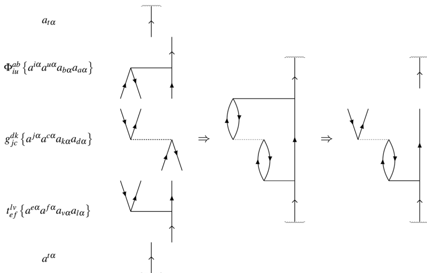
Fig. 2 Goldstone diagram construction representing the automated generation of the residual term r_{ab}^{iu} = g_{jc}^{dk} t_{ef}^{lv} \delta_k^i \delta_b^f \delta_a^c \delta_j^e \delta_d^e \delta_v^t .
