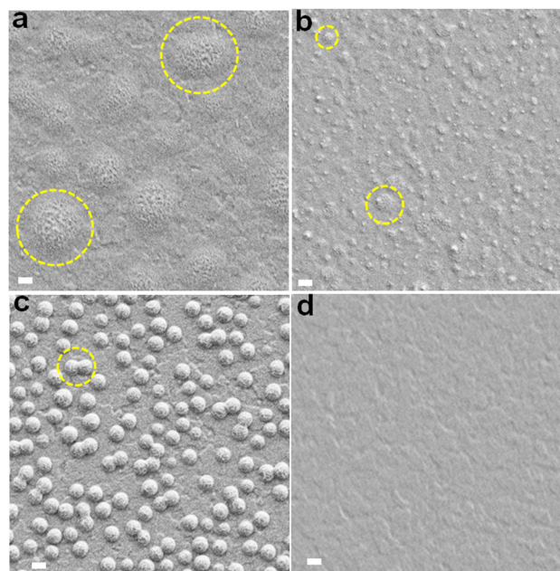
Fig. 2 SEM images ITO/bl-TiO 2 substrates after spin-coating DMF/DMSO dispersions (3.0 mg g -1 ) of (a) NG-60, (b) NG-100 and (c) NG-200 particles. An SEM of the bare ITO/bl-TiO 2 substrate is shown in (d) for comparison. The yellow circles highlight coalesced nanogels. Scale bars: 200 nm.
