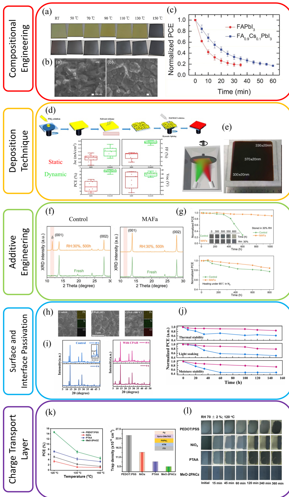
Fig. 9 General approaches reported in literature to improve performance and stability of \text{FAPbI}_3 perovskite solar cells. (a) \text{FAPbI}_3 and \text{FA}_{0.9}\text{Cs}_{0.1}\text{PbI}_3 films with different annealing temperatures, (b) Top view SEM images of \text{FAPbI}_3 and \text{FA}_{0.9}\text{Cs}_{0.1}\text{PbI}_3 and (c) normalized PCE of their respective solar cells without encapsulation measured over time in ambient. Cs incorporation resulted in formation of black perovskite even at room temperature. \text{FA}_{0.9}\text{Cs}_{0.1}\text{PbI}_3 has improved film quality and stability compared to pure \text{FAPbI}_3 . Reproduced with permission from ref. 69. Copyright © 2015 WILEY-VCH Verlag GmbH & Co. KGaA, Weinheim. (d) Schematic illustration of perovskite processing of \text{FAPbI}_3 solar cells processed with 2-step deposition method using dynamic
