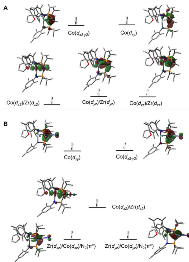
Fig. 7 Pictorial representations of the frontier MO diagrams of 7 (A) and 5 (B) derived from DFT calculations ( \omega B97XD/def2SVP).
