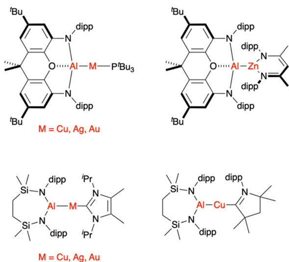
Fig. 1 Selected \text{Al-M} bonds known to insert \text{CO}_2 to form metallacarboxylates with C -bound M centres. 29,36–39 dipp = 2,6-di-isopropylphenyl.
