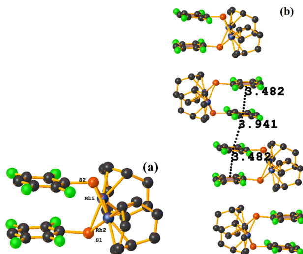
Fig. 47 (a) Molecular structure of JISSOT. (b) Supramolecular array of JISSOT.
