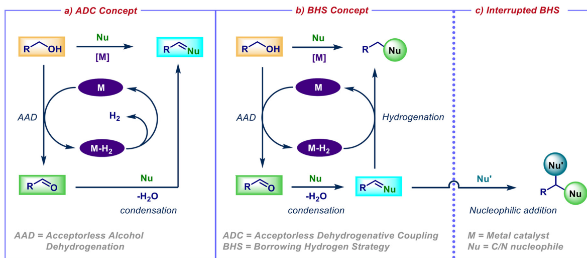
Fig. 2 Three main approaches to AAD reactions: (a) acceptorless dehydrogenative coupling (ADC), (b) borrowing hydrogenation strategy (BHS), and (c) interrupted borrowing hydrogen strategy.
