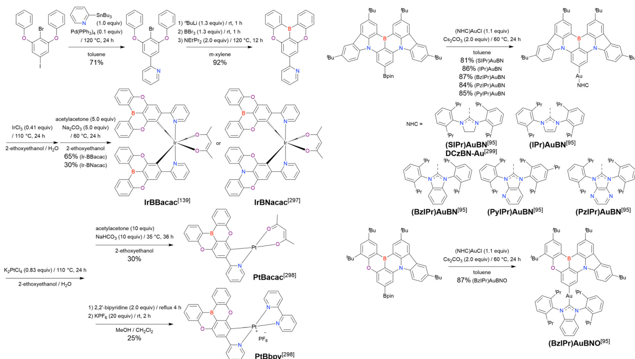
Scheme 51 Synthesis of DOBNA- and CznB-based metal complexes.
