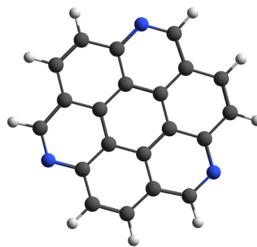
Fig. 1 Molecular structure of cationic 1,5,9-triazacorone ( \text{TAC}^{\bullet+} , \text{C}_{21}\text{H}_9\text{N}_3^{\bullet+} ).
