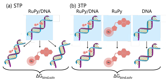
Fig. 5 Schematic representation of binding free energy calculation within the MM-PBSA approach with the (a) single trajectory protocol (STP) and (b) three trajectory protocol (3TP).
