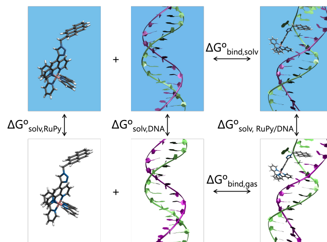
Fig. 4 Thermodynamic cycle scheme for binding free energy calculation with the MM-PBSA approach. Systems in white boxes depict gas phase, while systems in solvation are shown in blue boxes.
