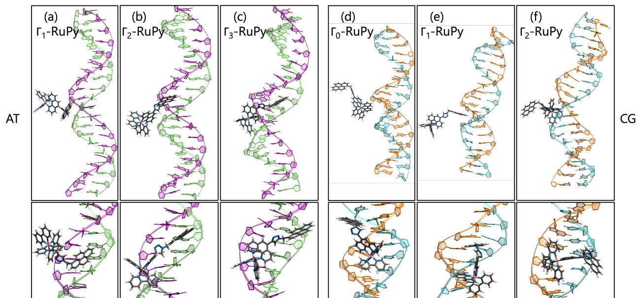
Fig. 10 Snapshots at time 100 ns in two different perspectives of the MD simulations with all \Gamma_i -RuPy with i = 0, 1, 2, 3 initially placed in the minor groove pocket of both poly(dA)poly(dT) and poly(dC)poly(dG) DNA double strands. Trajectories that converged to intercalative binding mode are not shown. Color code for atoms in RuPy and residues in DNA: grey for C, blue for N, pink for Ru, white for H, green for adenine, purple for thymine, light blue for cytosine, and orange for guanine.
