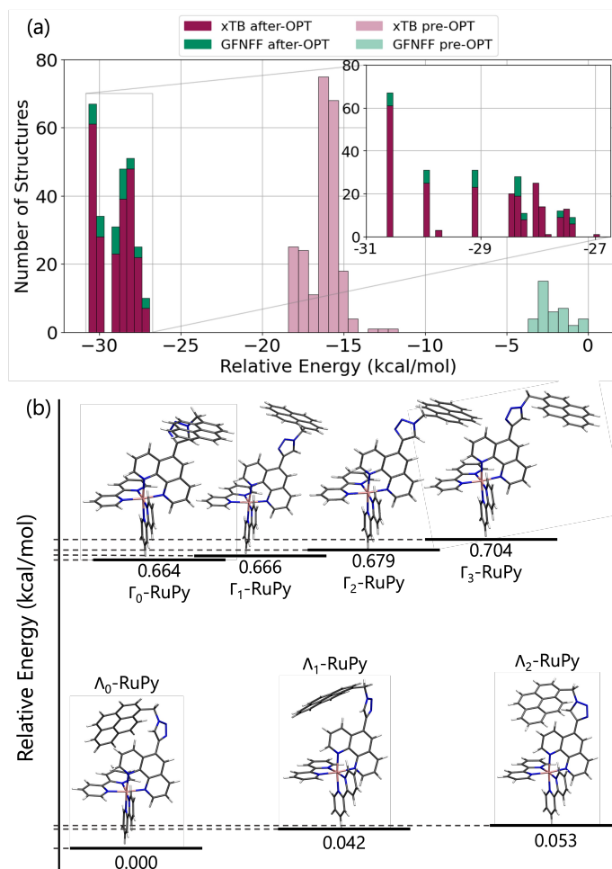
Fig. 6 (a) Histogram of relative single-point energies in kcal/mol calculated at the 3LYP-D3(BJ)/def2-SVP of theory in implicit water for RuPy geometries generated with CREST. In light pink and light green, the relative energy of the structures obtained with CREST at the xTB and GFNFF levels of theory, respectively. In dark pink and dark green, the relative energies after re-optimization at the B3LYP-D3(BJ)/def2-SVP level of theory. A zoom-up of the most stable re-optimized structures is also displayed. (b) Relative total energies in kcal/mol and geometries representation of the seven most stable clusters' representatives after CREGEN clustering algorithm. The reference corresponding to the lowest energy conformer is a \Lambda_0 -type of structure and has a total energy of -2550.67655 Hartree. The next two most stable –mostly degenerated– conformers are also \Lambda -shaped, followed by almost degenerated four \Gamma -shaped conformations.
