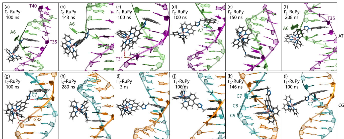
Fig. 9 Snapshots of the MD simulations with all \Gamma_i -RuPy with i = 0, 1, 2, 3 initially intercalated in both poly(dA)poly(dT) and poly(dC)poly(dG) DNA double strands. Color code for atoms in RuPy and residues in DNA: grey for C, blue for N, pink for Ru, white for H, green for adenine, purple for thymine, light blue for cytosine, and orange for guanine.
