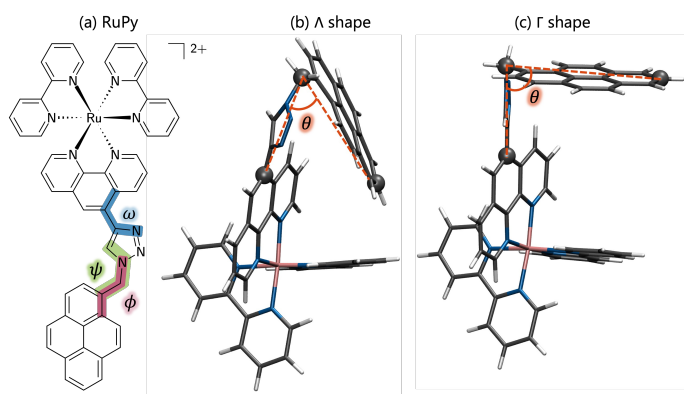
Fig. 1 (a) Structure of the ruthenium (II) complex (RuPy) depicting the \phi , \omega and \psi torsional angles in green, red and blue, respectively. (b) RuPy in the \Lambda -shaped geometry, and (c) \Gamma -shaped geometry. Color code for atoms and angle \theta : grey for C, blue for N, pink for Ru, white for H, and red for O.
