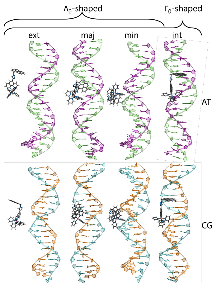
Fig. 7 Initial structures of RuPy/DNA adducts. \Lambda_0 -RuPy conformations were initially bound externally as well as in the major and minor grooves of AT and CG sequences (6 trajectories, 3 for each DNA sequence). \Gamma_0 -RuPy structures are additionally intercalated (8 trajectories, 4 for each DNA sequence).
