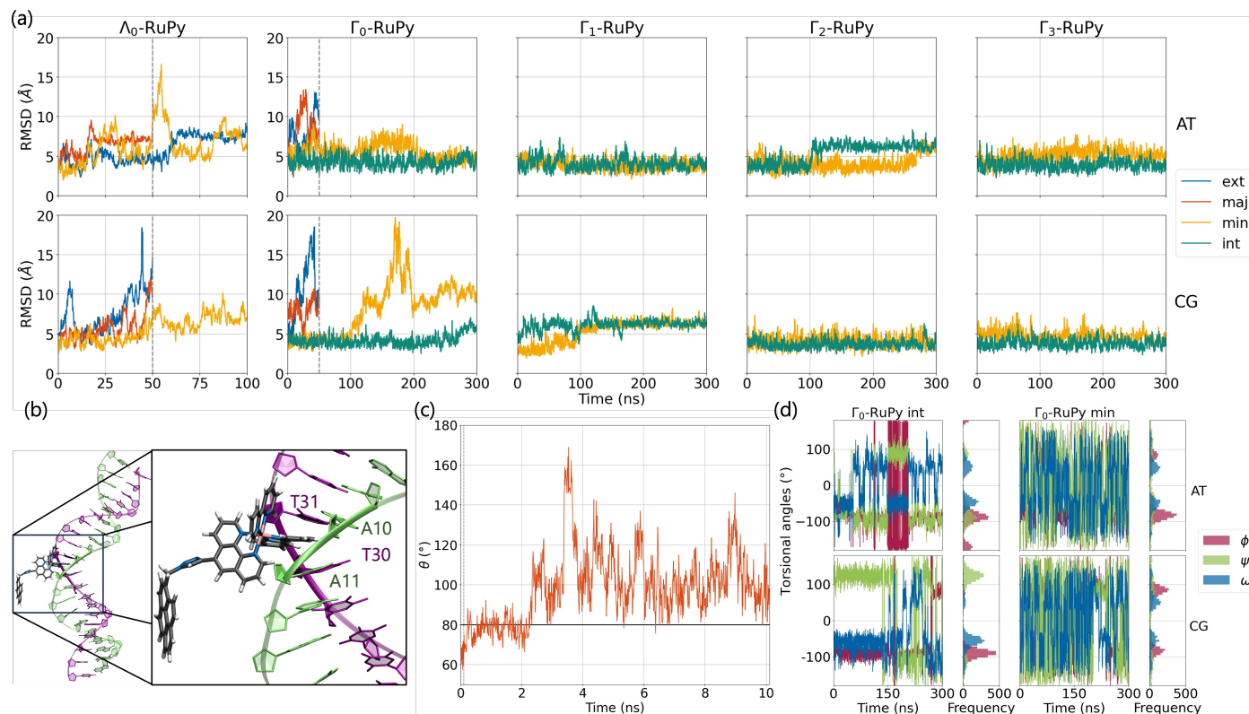
Fig. 8 (a) RMSD values of production run trajectories computed against the starting structures for \Lambda_0 -RuPy and \Gamma_i -RuPy with i = 0, 1, 2, 3 structures initially placed interacting externally (ext), in the major groove pocket (maj), in the minor groove pocket (min) or intercalated between two nucleobase pairs (int) of both poly(dA)poly(dT) (top) and poly(dC)poly(dG) (bottom) DNA double strands. (b) Partial intercalation of a bpy ligand of \Gamma_0 -RuPy between the nucleobase pairs A10-T31 and A11-T30. (c) Time evolution of angle \theta in the heating and equilibration stages of the simulation when \Lambda_0 -RuPy is initially placed in the major groove pocket of poly(dA)poly(dT) DNA double strand. The horizontal line at 80^\circ indicates the threshold for distinguishing between \Lambda -shaped geometry ( \theta < 80^\circ ) and \Gamma -shaped geometry ( \theta > 80^\circ ). (d) Time evolution and histogram of \phi , \psi and \omega torsional angles along the production runs for \Gamma_0 -RuPy initially placed in intercalated between two nucleobase pairs (int) and in the minor groove pocket (min) of both poly(dA)poly(dT) (top) and poly(dC)poly(dG) (bottom) DNA double strands.
