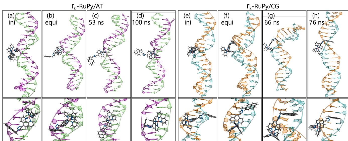
Fig. 11 Snapshots in two different perspectives of the MD simulation trajectory where (a-d) \Gamma_0 -RuPy was initially placed at poly(dA)poly(dT) minor groove pocket but evolved to intercalation of the bpy ligand and (e-h) \Gamma_3 -RuPy initially placed at poly(dC)poly(dG) minor groove pocket ends up intercalating by the pyrene moiety ligand. Color code for atoms in RuPy and residues in DNA: grey for C, blue for N, pink for Ru, white for H, green for adenine, purple for thymine, light blue for cytosine, and orange for guanine.
