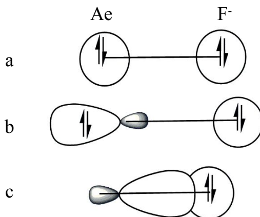
Fig.12: Schematic representation of the \sigma bond formation in \text{AeF}^- in three steps. (a) Initial charge distribution in \text{Ae} atom and \text{F}^- where the arrows indicate the total electronic charge; (b) Polarization of the valence electrons in \text{Ae} and (n)s^2 \rightarrow (n)s/p(\sigma) hybridization; (c) Concomitant formation of the vacant orthogonal (n)s/p(\sigma) orbital at \text{Ae} atom which overlaps with the occupied \sigma orbitals of \text{F}^- which leads to a polar covalent \text{Ae-F}^- bond.
