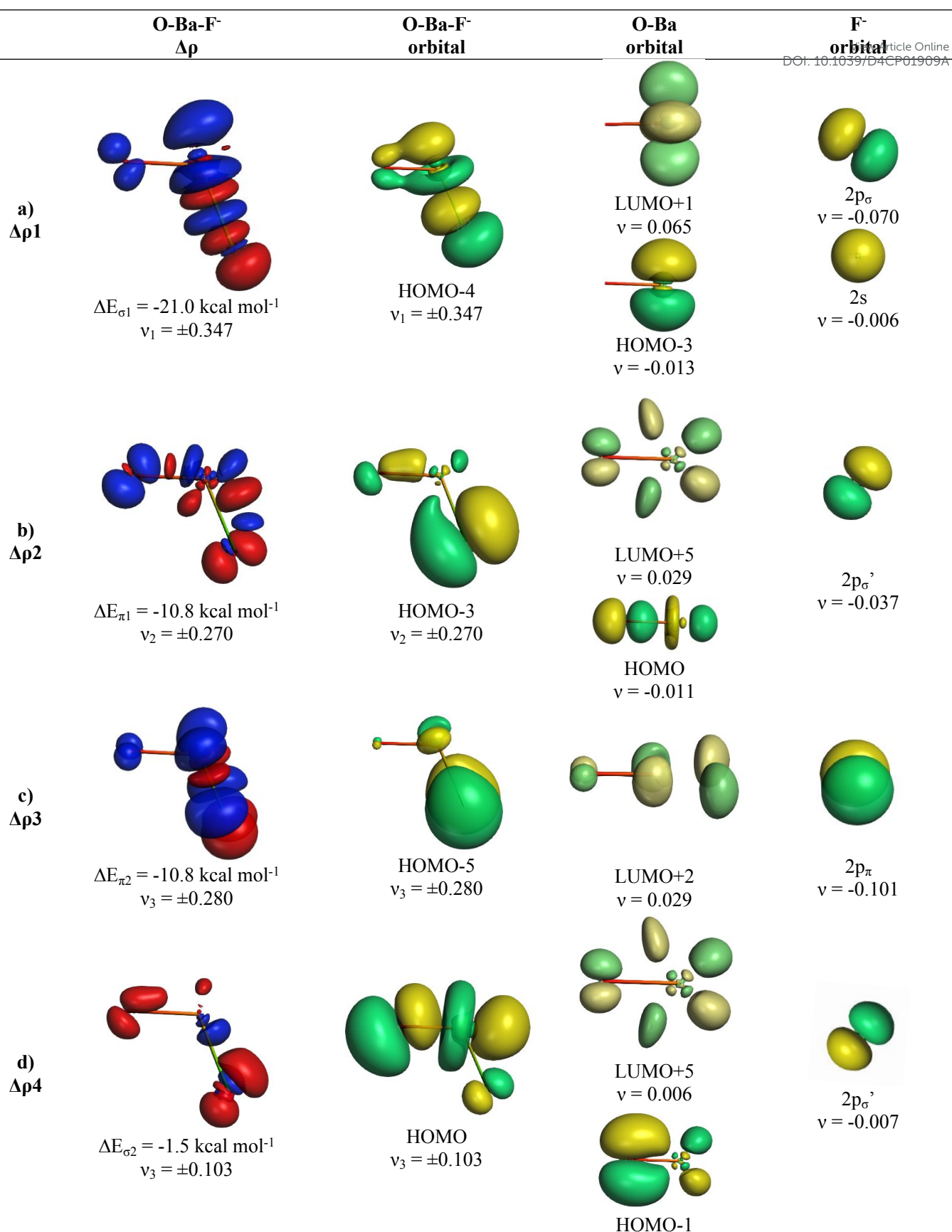
Figure 9. Plot of deformation densities \Delta\rho of OBaF - . The pairwise orbital interactions and the associated interaction energies ( \Delta E_{\text{orb}} ) between fragments OBa(S) and F - (S) in OBaF - of the bent equilibrium structure, as well as the shape of the most important interacting MOs. The direction of the charge flow is red→blue. (Isovalue 0.03e/au 3 ).
