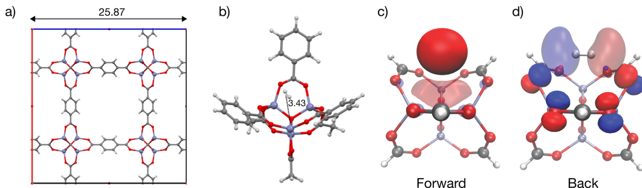
Fig. 5 Illustration of hydrogen binding at the cup site in MOF-5, a framework without open metal sites. (a) Cubic unit cell of MOF-5. (b) Cluster model for MOF-5 depicting relatively weak \text{H}_2 binding at the \alpha (cup) site, as implied by the long coordination distance. Dative contributions to \text{H}_2 binding are very weak in this dispersion-dominated interaction, consistent with the delocalized character of the framework acceptor and donor COVP orbitals shown in (c) and (d) together with the corresponding \text{H}_2 \sigma donor and \sigma^* acceptor orbitals. Distances are labelled in \text{\AA} with Zn(II) rendered in blue-grey, O in red, H in light grey and C in dark grey. The orbitals were plotted with an isosurface of \pm 0.07 \text{ \AA} . The smaller formate model was used to visualize charge transfer COVP orbitals.
