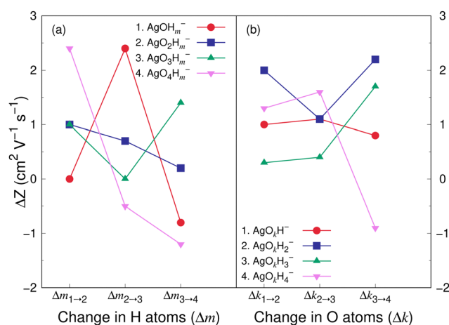
Fig. 9 Difference in electrical mobility, \Delta Z , (in \text{cm}^2 \text{V}^{-1} \text{s}^{-1} ) between (a) \text{AgO}_k\text{H}_{m-1}^- and \text{AgO}_k\text{H}_m^- clusters for k = 1-4 , and m = 2-4 ; (b) \text{AgO}_{k-1}\text{H}_m^- and \text{AgO}_k\text{H}_m^- clusters for k = 2-4 , and m = 1-4 . Z values of \text{AgO}_k\text{H}_m^- clusters have been calculated by the TM in helium carrier gas.
