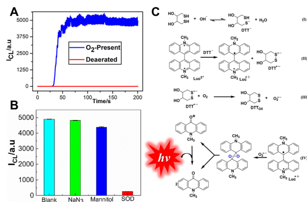
Fig. 6 (A) The effect of dissolved oxygen on the DTT/lucigenin system. Flow rate: 1.5 \text{ mL min}^{-1} ; [lucigenin]: 10 \mu\text{M} ; [DTT]: 0.3 \text{ mM} ; PMT voltage: -750 V. (B) Influences of radical scavengers on the DTT/lucigenin CL system. [lucigenin]: 0.1 \text{ mM} ; [DTT]: 0.3 \text{ mM} ; [ \text{NaN}_3 ]: 0.3 \text{ mM} ; [mannitol]: 0.3 \text{ mM} ; [SOD]: 0.5 \mu\text{g mL}^{-1} . 0.1 M PBS, pH 11. (C) CL mechanism of the DTT/lucigenin system. Reprinted with permission from ref. 45, Copyright 2022 American Chemical Society.
