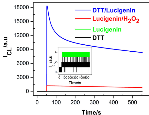
Fig. 5 CL intensity versus time profiles for the systems of lucigenin/DTT, lucigenin/ \text{H}_2\text{O}_2 , lucigenin, and DTT. Inset: enlarged CL emissions of DTT and lucigenin. [lucigenin]: 0.1 mM; [DTT]: 1.0 mM; [ \text{H}_2\text{O}_2 ]: 1.0 mM; 0.1 M PBS (pH 11); PMT voltage: -750 V. Reprinted with permission from ref. 45, Copyright 2022 American Chemical Society.
