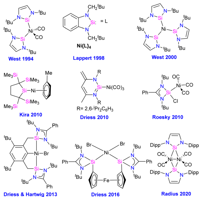
Fig. 12 Selected examples of \text{Ni} complexes of silylenes.
