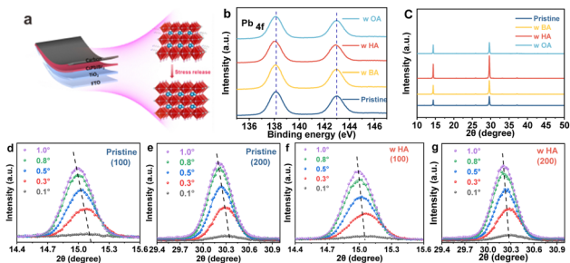
Fig. 1 (a) Schematic diagram of stress control. (b) Pb 4f XPS spectra of perovskite films. (c) XRD and (d)–(g) depth-dependent XRD patterns of perovskite films.
