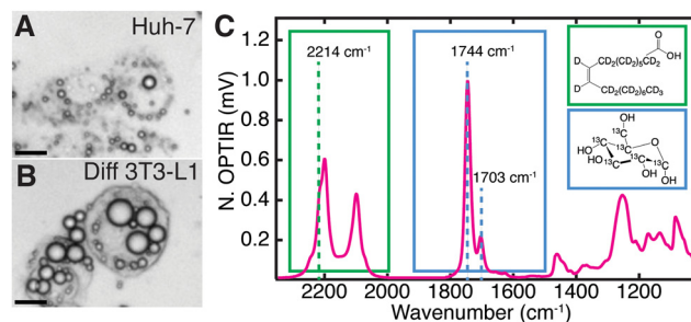
Fig. 2 Live cell characterization of the cell lines (A) Huh-7 and (B) differentiated 3T3-L1 after feeding with ^2\text{H} oleic acid ( 60\ \mu\text{M} ) and ^{13}\text{C} glucose ( 4.5\ \text{mg mL}^{-1} ). Scale bars are 20\ \mu\text{m} . (C) Full IR spectra of a point within a fixed Huh-7 cell LD 48 hours after feeding ^2\text{H} OA. ^2\text{H} -C from the ^2\text{H} oleic acid (green, structure in inset) which has been esterified in LDs. 2214\ \text{cm}^{-1} is assigned to ^2\text{H} -C stretching. ^{13}\text{C}=\text{O} stretch at 1703\ \text{cm}^{-1} where the ^{13}\text{C} comes from metabolized ^{13}\text{C} glucose (blue, structure in inset). Pictured alongside the unlabelled ^{12}\text{C}=\text{O} band at 1744\ \text{cm}^{-1} .
