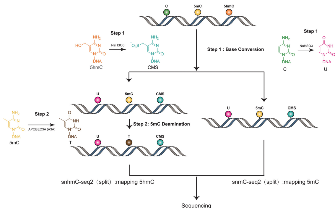
Fig. 3 Overview of Joint-snmC-seq. The figure demonstrates the concurrent profiling of 5mC and 5hmC at the single-cell level.
