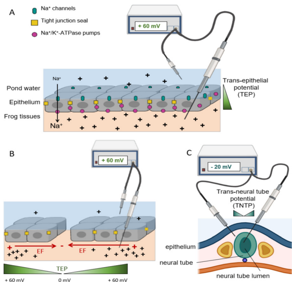
Fig. 1 Structurally polarised epithelial cells, in which \text{Na}^+ channels are restricted to apical cell membrane surfaces (pond water side) and the \text{Na}^+/\text{K}^+/\text{ATPase} pumps are localised to the basolateral cell membranes (frog tissue side). Neighbouring cells are fastened to each other by tight junctions, which provide a high resistance epithelial seal and they also aid physical segregation of ion pumps and channels in apical and basal membrane domains, respectively. Net inward movement of \text{Na}^+ ions creates an internally positive transepithelial potential difference (TEP) relative to the pond water of about +60 mV. (B). Upon wounding, the \text{Na}^+ ions leak out of the wound, collapsing the TEP to 0 mV at the injury, but distal to the wound (intact epithelium) the inward ion flow is uninterrupted, so the TEP remains +60 mV. The resulting potential difference between the wound site and intact tissues generates an electric field (red arrow) parallel to the epithelial layer, with the wound centre as a cathode (negative). The green wedge indicates the TEP gradient within tissues. (C) The embryonic neural tube, which is the precursor to the brain and spinal cord, maintains a potential difference of about -20 mV across itself. It forms from folds of the outer layer of the embryo, so its inside lumen shares ion transport traits with apical frog skin. Consequently, the lumen is negative relative to the tissues just outside the neural tube. Extracted from ref. 3 under Creative Commons License.
