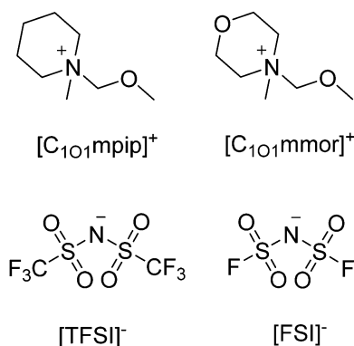
Fig. 1 Structure and abbreviations of cation and anions used. Cation abbreviations are: N -methoxymethyl- N -methylpiperidinium [C 101 mpip] + and 4-methoxymethyl-4-methylmorpholinium [C 101 mmor] + . Anion abbreviations are bis(trifluoromethanesulfonyl)imide [TFSI] − , and bis(fluorosulfonyl)imide [FSI] − .
