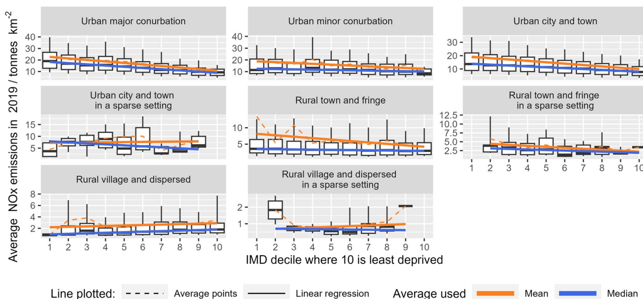
Fig. 5 The relationship between IMD decile and average \text{NO}_x emissions for each rural urban classification (RUC) in England.
