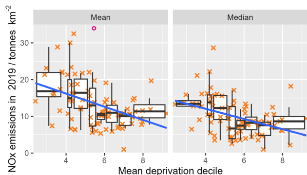
Fig. 4 Scatter plot linking the average total \text{NO}_x emission and mean IMD decile for all counties and unitary authorities in England. Counties and unitary authorities within London are omitted. The blue line is the line of best fit for linear regression using all points plotted. Each cross in orange represents a single county or unitary authority. The boxplot is split into 8 bins containing equal numbers of counties/unitary authorities and uses standard procedures for plotting the whiskers. The circular point in pink has an emission of 42 tonnes per \text{km}^2 .
