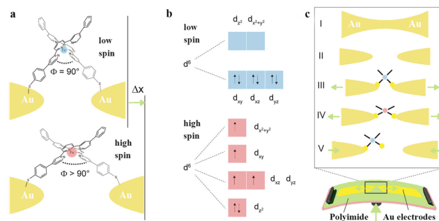
Fig. 6 Two-terminal mechanically controlled single-molecule junctions. (a) Sketch of the \text{Fe}^{\text{II}} -based spin-crossover molecular junction in the ideal arrangement to trigger the LS to HS switch by separating the electrodes by \Delta x . (b) Iron II 3d levels involved in the spin-crossover phenomenon. (c) Schematic illustration of a mechanically controllable break junction (MCBJ) setup (bottom) with the molecule placed in the junction. Reproduced with permission. 42 Copyright 2016, American Chemical Society.
