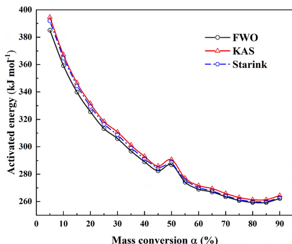
Fig. 9 Activation energy ( E_a ) of a [N_{4444}][NTf_2] at different degrees of conversion.
