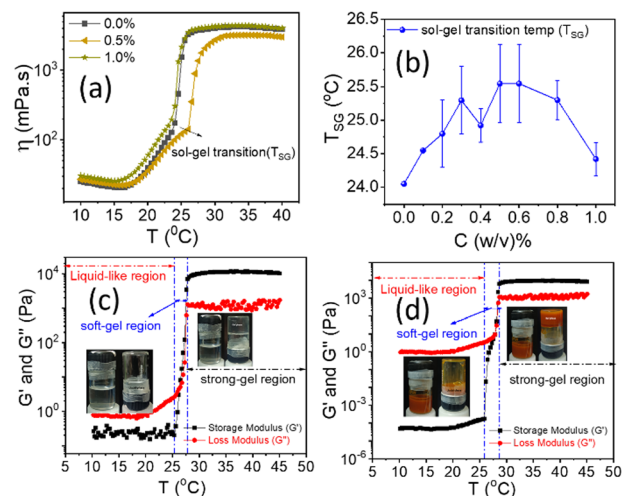
Fig. 7 (a) Temperature sweeps at a constant shear rate ( \dot{\gamma} = 50 s −1 ) of the composite system at various NR concentrations. (b) The sol–gel transition temperature is plotted as a function of \beta -FeOOH NR concentrations in 20% PF127 (c) oscillatory temperature sweep, with temperature-dependent storage ( G' ) and loss ( G'' ) moduli at a fixed angular frequency ( \omega = 10 rad s −1 ) and shear strain ( \gamma ) = 0.1% for only 20% PF127 and (d) temperature sweep for the composite of 20% PF127 with 0.4% \beta -FeOOH NRs. Here we define 3 regions: first, the liquid-like region, where G'' is dominated over G' , second, the soft-gel region, where G' is dominated over G'' , and third, the strong-gel. Solid lines are a guide to the eye.
