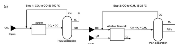
Fig. 19 Process diagram of the tandem HT CO 2 electrolysis to CO and LT CO electrolysis towards C 2 H 4 , the so-called tandem process. Adapted from Sisler et al. , 2021. 51
