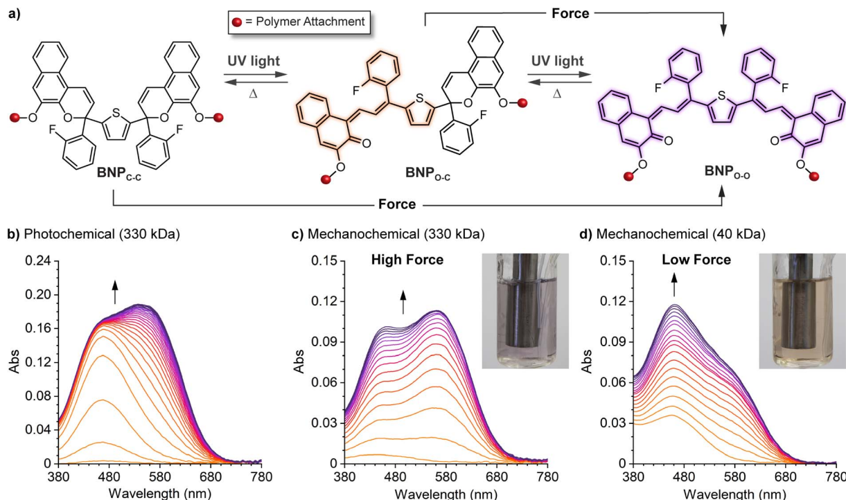
Fig. 12 Force-dependent multicolor mechanochromism from a bis-naphthopyran (BNP) mechanophore. (a) Unlike the sequential ring-opening reactions observed upon photochemical activation, mechanical force directly converts the BNP mechanophore to the purple bis-merocyanine species, which thermally reverts to the yellow monomerocyanine. Changing the amount of force delivered to the mechanophore biases the merocyanine distribution resulting in force-dependent coloration. (b) UV-vis absorption spectra of a 330 kDa poly(methyl acrylate) polymer with a chain-centered BNP unit illustrating sequential-ring opening behavior upon irradiation with UV light. Ultrasound-induced mechanochemical activation of (c) the same 330 kDa polymer, and (d) an analogous 40 kDa polymer that experiences lower force, illustrating non-sequential ring opening behavior. Insets show photographs of the final sonicated solutions. Adapted with permission from ref. 135. Copyright 2019, American Chemical Society.
