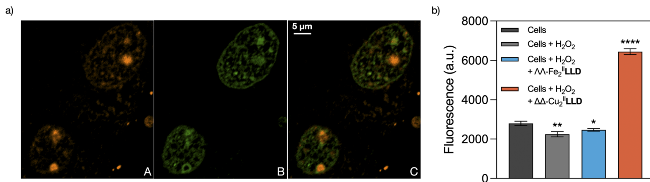
Fig. 6 (a) \Delta\Delta -Cu II 2TAMRA-LLD selectively stains DNA replication sites at the cell nuclei. Vero cells expressing protein GFP-PCNAL2 were incubated in the presence of 25 \mu g mL -1 of digitonin for 3 min and then in the presence of 5 \mu M of \Delta\Delta -Cu II 2TAMRA-LLD for 15 min. The Cu II peptide helicite used in these studies was previously assembled before the internalization experiment by adding 5 eq. of CuCl 2 ·2H 2 O to an aqueous solution of TAMRA-LLD peptide ligand. (A) Red channel emission showing the distribution of the TAMRA-labelled helicite; (B) green channel, corresponding to the emission of the GFP-PCNAL2 probe that labels DNA replication foci; (C) overlay of the green and red channels, which shows that \Delta\Delta -Cu II 2TAMRA-LLD has localised at the replication foci. Nucleoli are clearly labelled as red spots inside the cell nuclei. The images show a representative confocal section of the Vero cells. (b) Detection of free DNA ends by TUNEL assay. S-phase synchronized Vero cells were incubated with H 2 O 2 alone and with \Lambda\Lambda -Fe II 2LLD or \Delta\Delta -Cu II 2LLD plus H 2 O 2 at 37 °C for 2 hours and then subjected to TUNEL analysis for the detection of free DNA ends. Results are represented as the mean with standard deviation of a triplicate experiment * = P \leq 0.05 ** = P \leq 0.01 *** = P \leq 0.001 and **** = P \leq 0.0001 .
