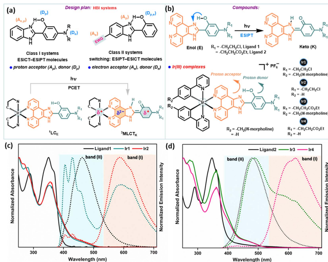
Fig. 2 (a) Design plan for synthesizing desired compounds. (b) Structures of phenanthroline-BIP based ancillary ligands attributing to the ESIP+PCET (ET-PT) phenomenon and the corresponding Ir(III)-complexes. The proton-accepting and donating parts are indicated in orange and cyan dark colors, respectively. (c) and (d) Normalized UV-vis absorption spectra (solid line) and the corresponding emission spectra (dotted line) of (c) ligand1, Ir1 and Ir2; (d) ligand2, Ir3 and Ir4; in DCM (10 \mu M), respectively under 365 nm excitation. Two emission bands are assigned as major band (I) and minor band (II), respectively.
