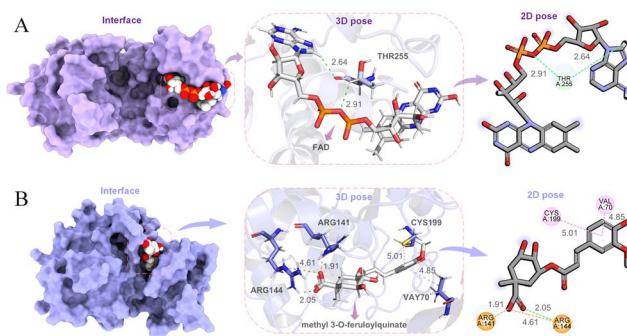
Fig. 12 Binding of potential lead compounds to targets. (A) Docking interface, 3D pose, and 2D pose of the PGK1-FAD complex. (B) Docking interface, 3D pose, and 2D pose for methyl 3-O-feruloylquininate docking with GSK3 \beta .
