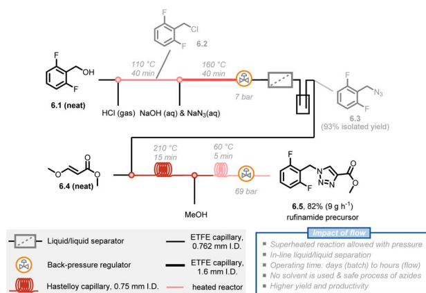
Fig. 6 Schematic representation of a 5-stage multi-step flow synthesis of a rufinamide precursor under superheated conditions. ETFE: ethylene tetrafluoroethylene.
