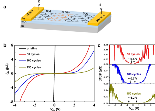
Fig. 3 (a) The illustration of a typical SLG/SLGBr/SLG diode. (b) The I_{ds} - V_{ds} curves of SLG/SLGBr/SLG diodes with different degrees of bromination. (c) The corresponding differential conductance dI/dV as a function of V_{ds} for the diodes.
