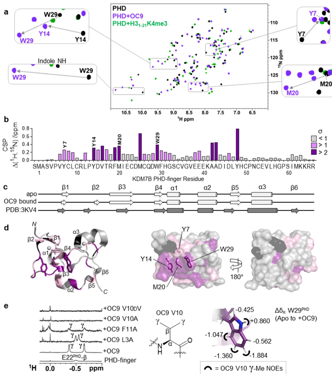
Fig. 4 Protein NMR reveals valine contacting the aromatic cage. (a) ^1\text{H} - ^{15}\text{N} HSQC of KDM7B PHD-finger in the apo (black) or bound forms with OC9 (purple, 1 : 1) or H31-21K4me3 (green, 3 : 1). (b) ^1\text{H} and ^{15}\text{N} chemical shift changes for apo vs. + OC9 were combined and weighted to give chemical shift perturbation (CSP) ( \Delta\delta ) values. Standard deviation ( \sigma ) of \Delta\delta are indicated (>1 pink, >2 purple). (c) TALOS+ predicts similar secondary structure elements in apo and OC9-bound solution protein complexes (light grey) to those found in PDB ID 3KV4 (dark grey). (d) Mapping of CSP \sigma from (b) onto PDB ID 3KV4 shows OC9 binding surfaces primarily along one face, which presents the cage (annotated residues). (e) Shielded ^1\text{H} -NMR signals centred around -0.5 ppm belonging to the OC9 V10 \gamma -methyl groups are observed in some OC9-PHD complexes, but not in apo protein, or complexes with OC9 V10A and OC9 V10DV. The V10 OC9 \gamma -methyl signals have NOE interactions (black semi-circles) with the W29 PHD indole, which itself is shielded upon binding of OC9 (indicated by \Delta\delta_{\text{H}} values).
