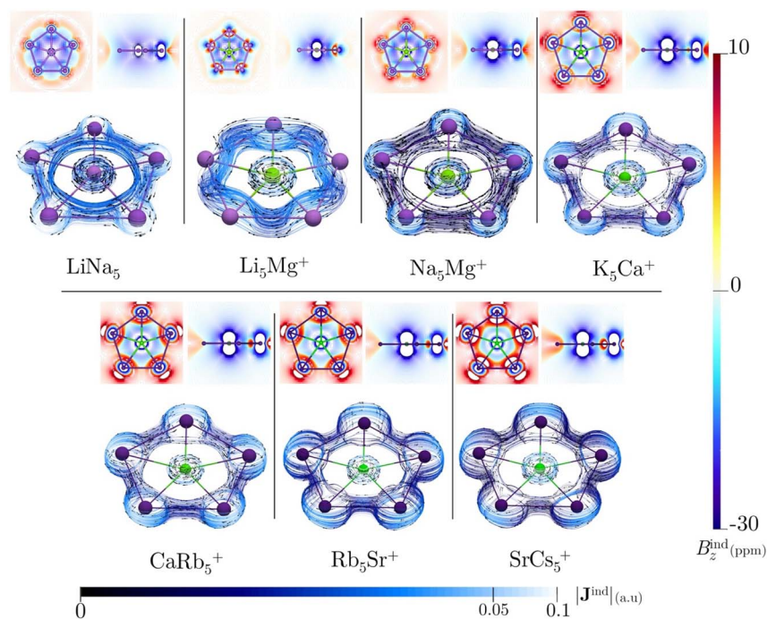
Fig. 3 In the top panel: the B z ind isolines plotted in the molecular plane (left) and a transversal slice (right). In the bottom panel: J ind maps plotted near the molecular plane. The arrows indicate the direction of the current density. The |J ind scale is in atomic units (1 au = 100.63 nA T −1 Å −2 ). The external magnetic field is oriented parallel to the z -axis, perpendicular to the molecular plane.
