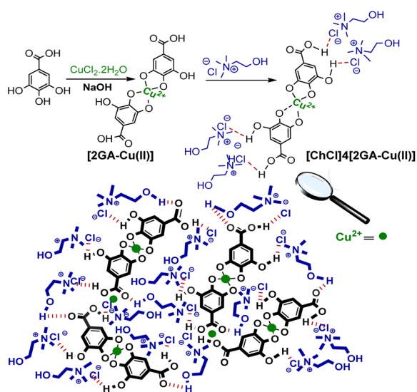
Scheme 2 The suggested illustration of molecular structure of [\text{2GA-Cu(II)}] complex and also possible interactions between [\text{2GA-Cu(II)}] complex and choline chloride ( \text{ChCl} ).
