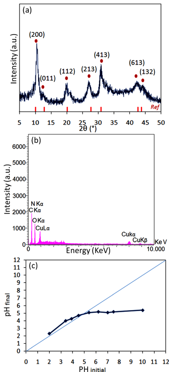
Fig. 2 (a) Powder X-ray diffraction of [\text{2GA-Cu(II)}] ; (b) EDX analysis of [\text{2GA-Cu(II)}] ; (c) \text{pH}_{\text{pzc}} determination graph of [\text{2GA-Cu(II)}] .
