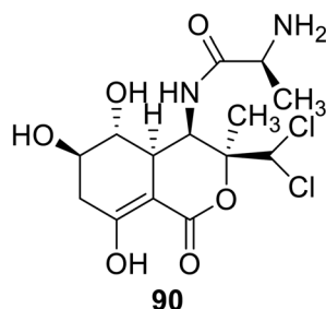
Scheme 11 Synthesis of bactobolin A 90.
