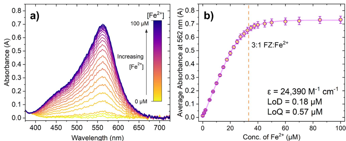
Fig. 2 (a) Absorbance spectra of ferrozine ( 100\text{ }\mu\text{M} ) in pH 5.6 MES buffer (0.1 M) with increasing concentration of \text{Fe}^{2+} ions. Note that this spectrum shows an example of one repeat, and three repeats were taken overall. (b) The average absorbance at the maximum (562 nm) taken over three repeat measurements, with error bars showing standard deviation. The dashed orange line indicates the concentration of \text{Fe}^{2+} at which the 3 : 1 FZ: \text{Fe}^{2+} complex is expected to form (approx. 33.33\text{ }\mu\text{M} \text{Fe}^{2+} ). Data fitted using a biphasic dose response function in OriginPro®.
