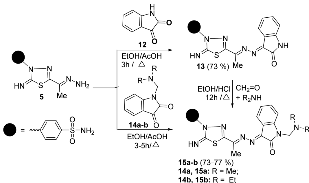
Scheme 3 Reaction of aminohydrazone 5 with heterocyclic ketones 12 , 14a – b .
