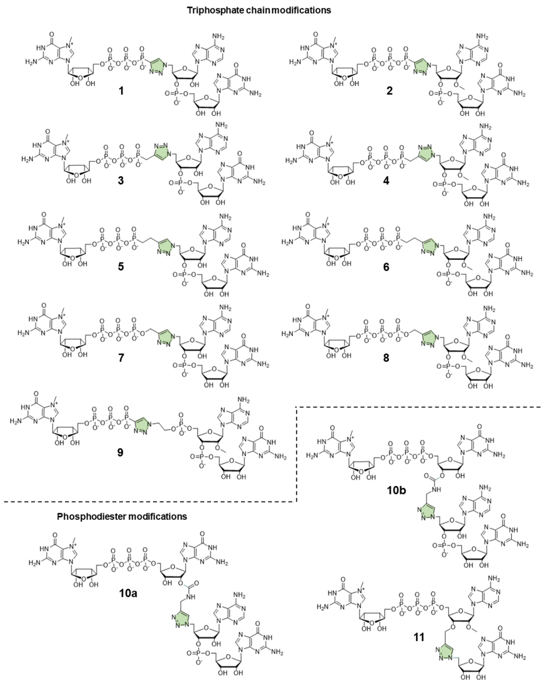
Fig. 2 Structures of phosphotriazole trinucleotide cap analogs synthesized in this work.
