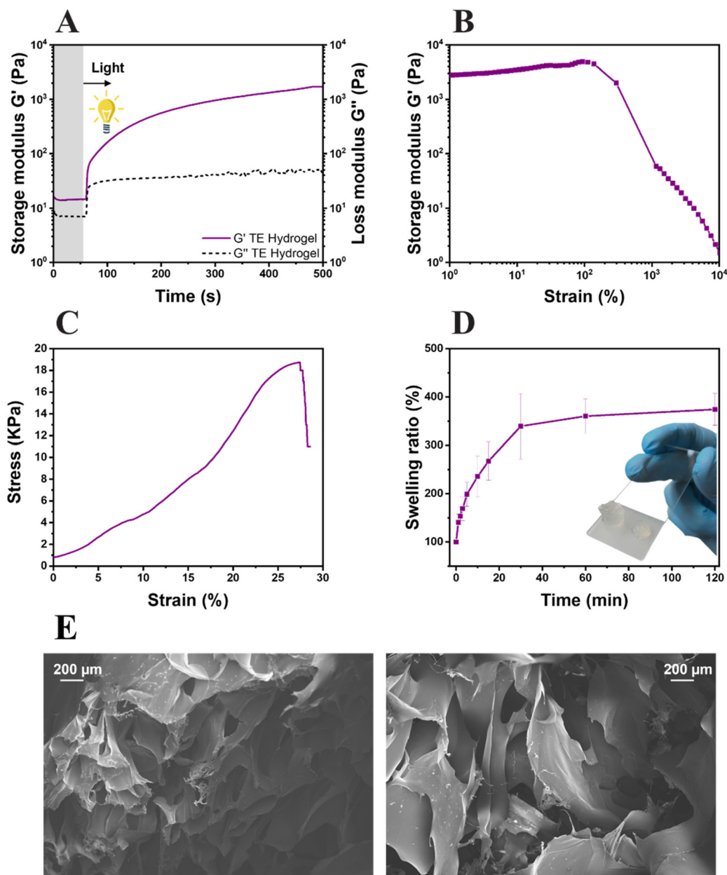
Fig. 4 Photoreology (A), amplitude sweep (B), compression test (C) and swelling kinetics (D) of the thiol–ene hydrogel (TE hydrogel). Field Emission Scanning Electron Microscopy (FESEM) of the TE hydrogels; scale bar 200 \mu\text{m} (E).
