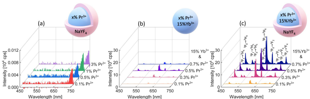
Fig. 2 Anti-Stokes emission spectra of \beta -NaF 4 nanocrystals: (a) core–shells singly doped with Pr 3+ ions; (b) cores co-doped with x\%Pr^{3+} , 15%Yb 3+ ; (c) x\%Pr^{3+} , 15%Yb 3+ co-doped cores with a passive shell with assigned transitions. The presented emission spectra were recorded under 852 nm excitation (1.5 MW cm -2 ) at room temperature.
