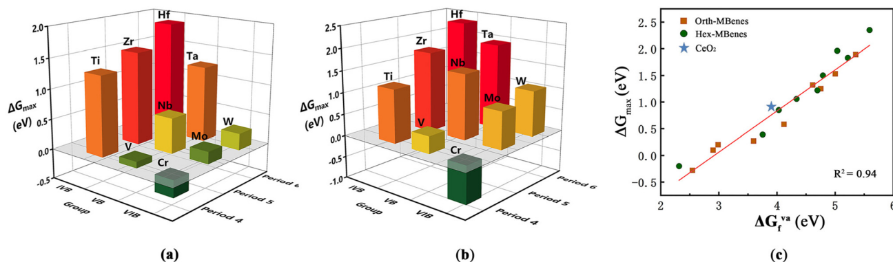
Fig. 5 \Delta G_{\max} for COOR of (a) orth- M_2B_2O_2 and (b) hex- M_2B_2O_2 with M in different groups and periods. (c) Relationship between \Delta G_{\max} and \Delta G_f^{Va} of orth/hex- M_2B_2O_2 .
