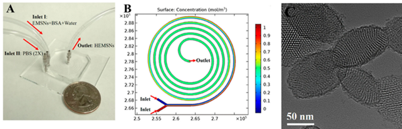
Fig. 13 A) Microfluidic chip for the fabrication of EMSNs. (B) COMSOL simulation result of mixing in the microfluidic spiral channel, and their morphologies. Reprinted from ref. 142.
