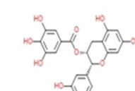
Epigallocatechin 3-O-gallate [3]
