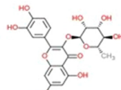
Quercetin 3-O-rhamnoside [1]
