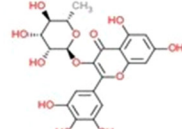
Myricetin 3-O-rhamnoside [1]
