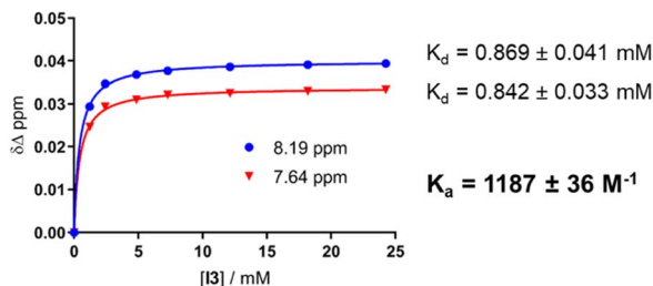
Fig. 9 Titration curve correlating the changes in the chemical shifts of aromatic protons in T_L1 with the changes in the concentration of I during the titration (left); K_d values obtained for both fits and the average K_a value (right).
