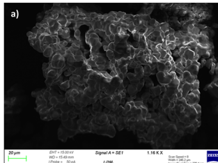
Fig. 5 SEM images of \text{Li}_2\text{MoO}_4 – pristine (a) and ball milled (b).
