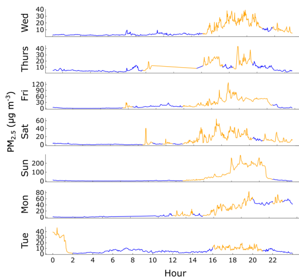
Fig. 8 \sigma_{\Delta PM} filter applied to unit ccc9 for the first week in December 2021. Blue data points correspond to periods of low \sigma_{\Delta PM} , yellow data points correspond to periods of high \sigma_{\Delta PM} .
