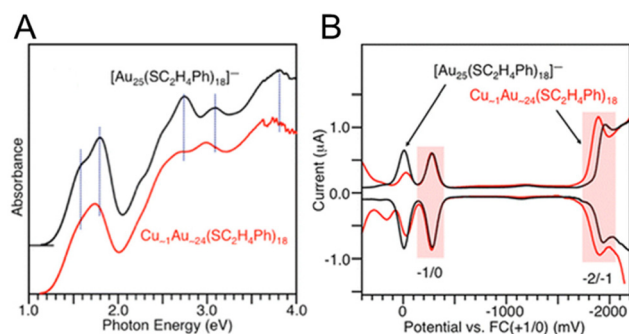
Fig. 10 (A) Optical absorption spectra of \text{Cu}_{1.1}\text{Au}_{24.9}(\text{PET})_{18} and [\text{Au}_{25}(\text{PET})_{18}]^- . The dotted lines indicate the main peak positions in the absorption spectrum of [\text{Au}_{25}(\text{PET})_{18}]^- . (B) DPV curves of \text{Cu}_{1.1}\text{Au}_{24.9}(\text{PET})_{18} and [\text{Au}_{25}(\text{PET})_{18}]^- . The red shaded regions indicate the peaks derived from the redox potentials of -2/-1 and -1/0 . Reproduced with permission from ref. 111. Copyright 2012, American Chemical Society.
