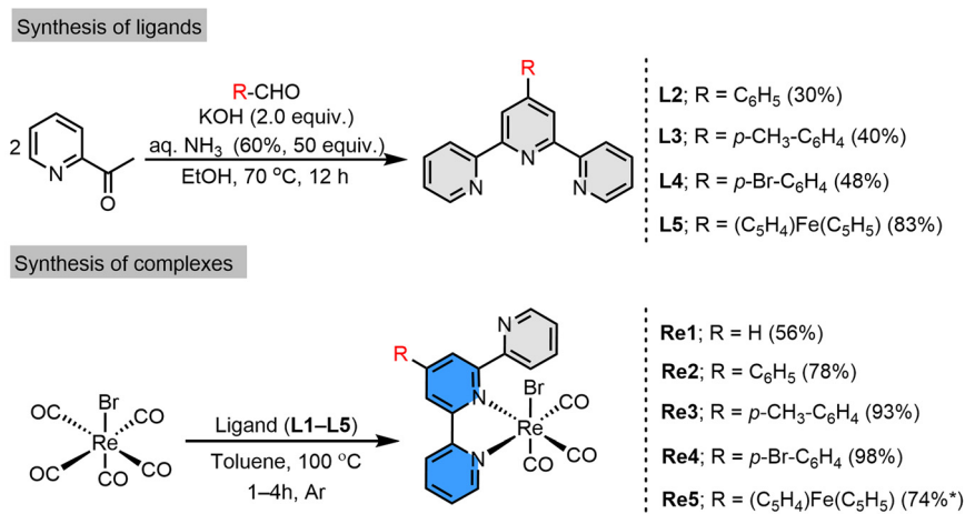
Scheme 1 Synthesis of terpyridine ligands (L2–5) and fac - \text{Re}(\text{i})(\text{L})(\text{CO})_3\text{Br} complexes ( Re1–5 ), where L = L1–5. * Re5 contains toluene (~0.5 molecules, calculated from ^1\text{H} NMR) as a solvent of crystallisation.
