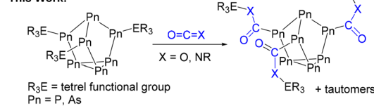
Fig. 1 Previously reported reactions of [\text{Pn}_7] clusters with small molecules and this work.
